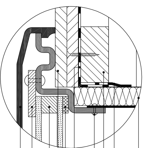
DETAIL I
